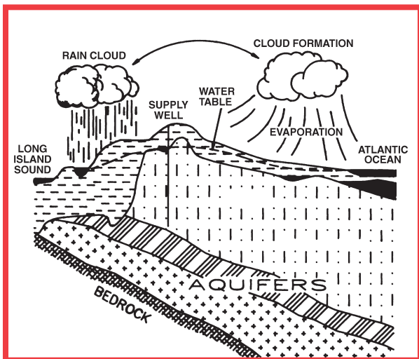
Aquifer System
